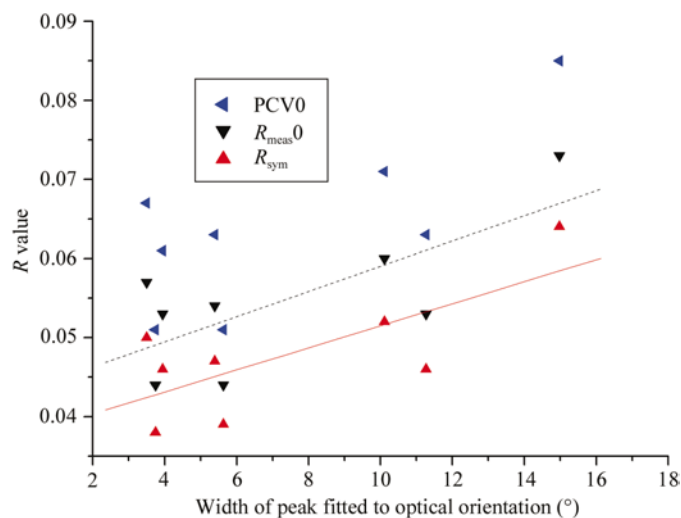
Figure 10 Plot of R_{\text{sym}} , R_{\text{meas}0} and the pooled coefficient of variation (PCV0) against the width of the fitted optical peak for eight glucose isomerase crystals. The trend lines for R_{\text{sym}} (red, continuous) and R_{\text{meas}0} (black, dashed) are shown.
