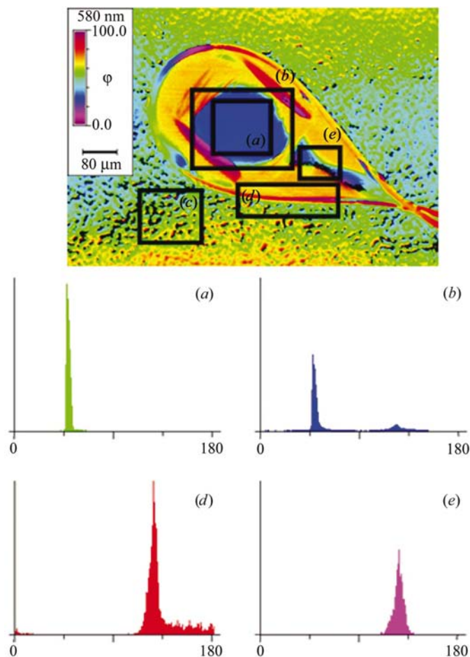
Figure 6 Illustration of the different peaks obtained from a typical orientation ( \varphi ) image. A threshold of \sin \delta \geq 0.1 was set for all the peak analyses. It can be seen that the ordered region of the crystal results in a sharp peak as in (a) and (b). After a threshold of 0.1 was set no data remained in region (c), so it is not plotted. The loops in which the crystals are mounted are birefringent, so selection of region (d) also results in a sharp peak. The area used for analysis was chosen such that the loop did not contribute to the peak fitted to the crystal data. Disordered regions such as the solvent produce broader peaks (e).
